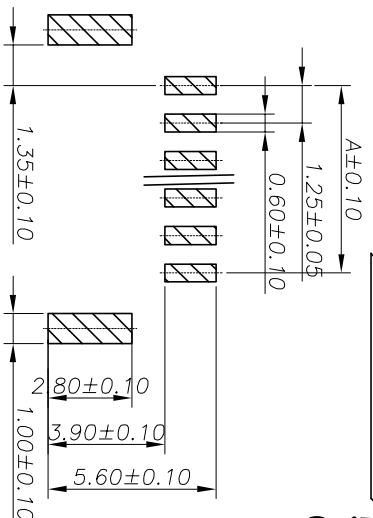
PCB Layout
