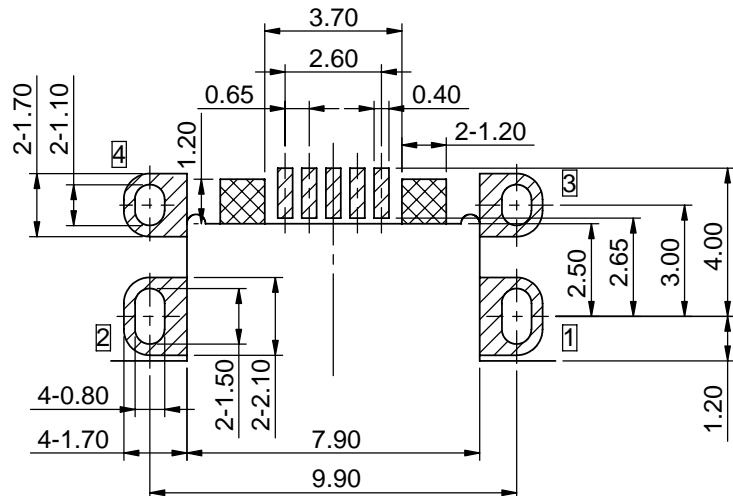
RECOMMENDED PCB LAYOUT(TOP VIEW) T=0.80mm (GENERAL TOLERANCE ±0.05)
