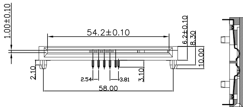
SEC. C-C
